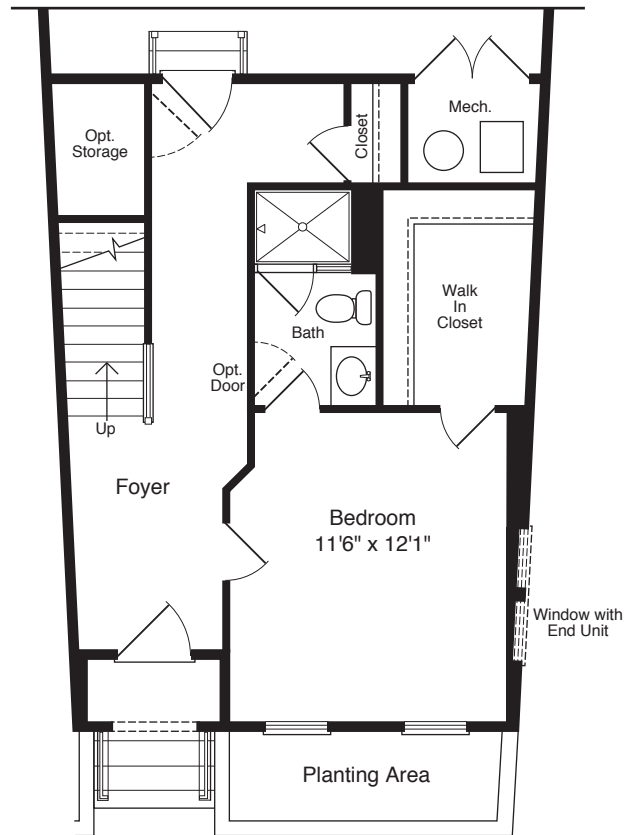
The Astra Partial Ground Floor Plan w/ Bedroom & Bath
