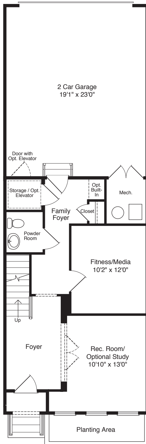
The Luna Ground Floor Plan Window Patterns Vary By Elevation
